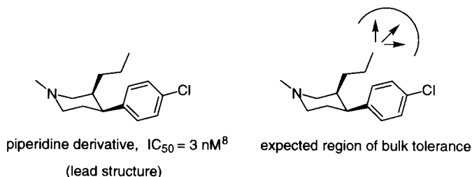
Figure 2. Piperidine derivative with high binding affinity to the DAT and expected region of bulk tolerance.
