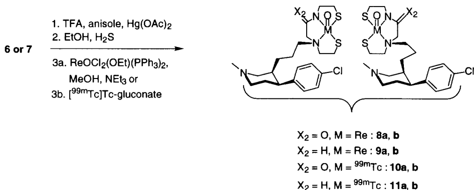
Scheme 2. Preparation of the rhenium/technetium complexes 8 , 9 , 10 , and 11 .
