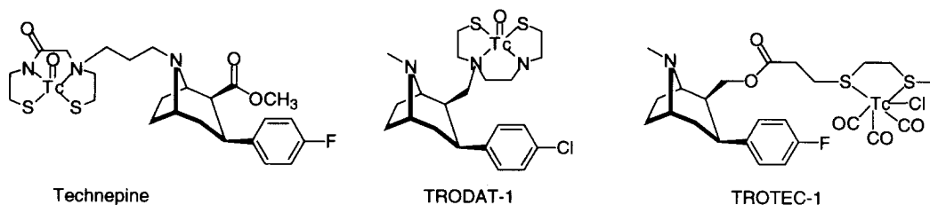
Figure 1. Tropane technetium conjugates.
